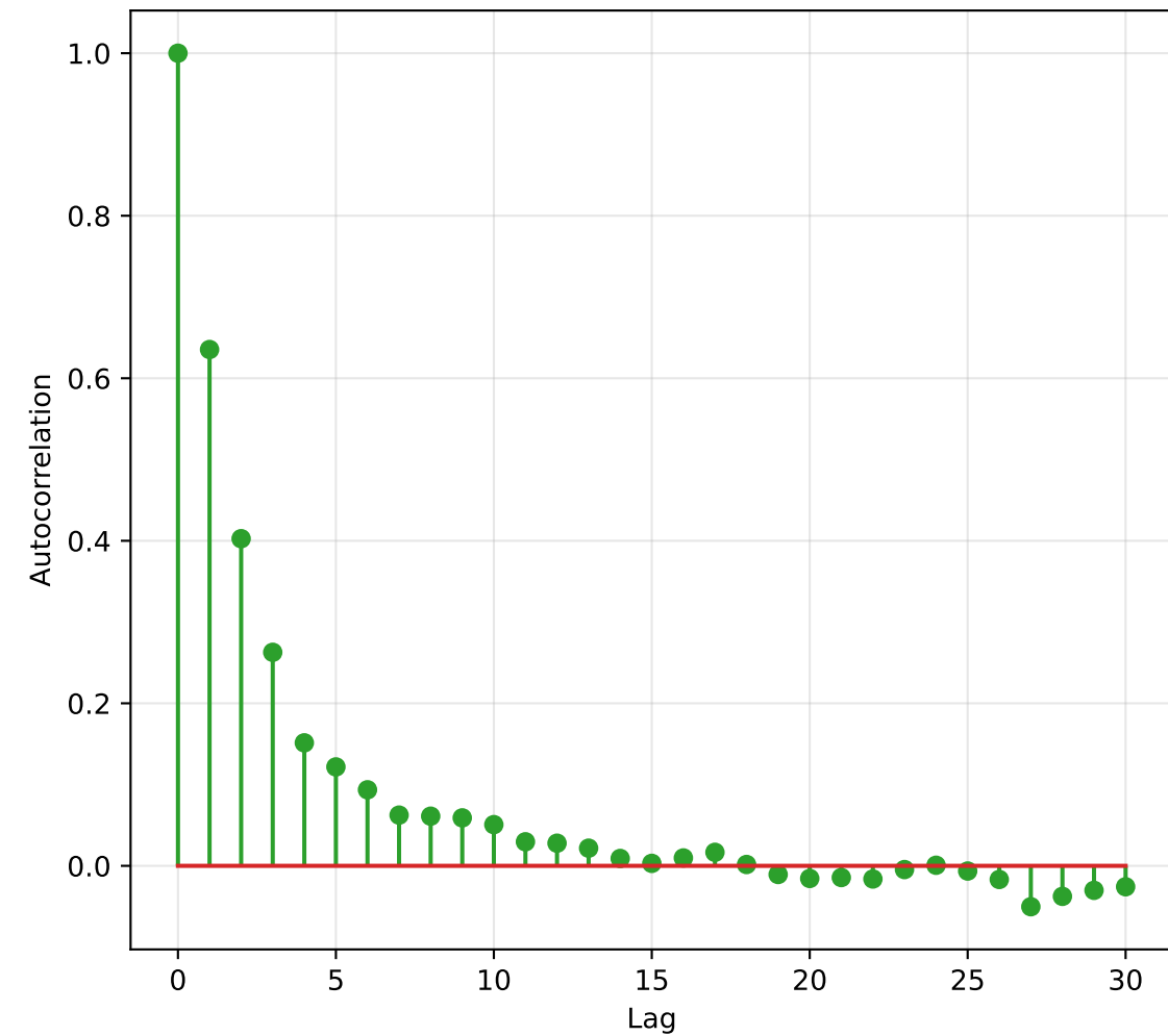
Autocorrelation: Normal
