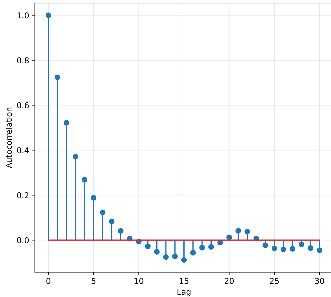
Autocorrelation: Uniform
